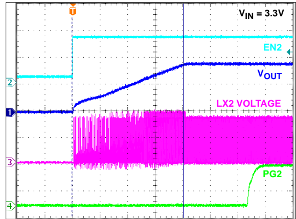
FIGURE 18. SOFT-START WITH NO LOAD CHANNEL 2
